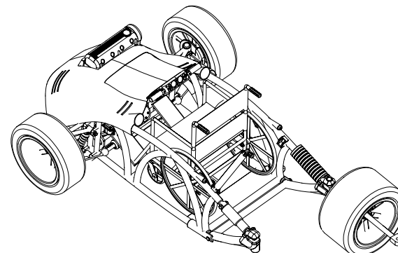
Wheel chair, belts in and starts to close until axel latches
