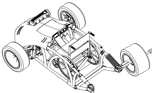
Wheel chair, belts in and starts to close until axel latches
