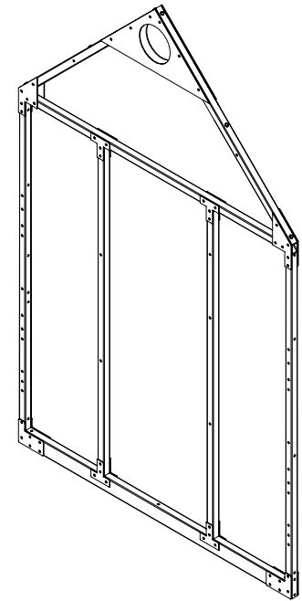
Frame assembly 1
