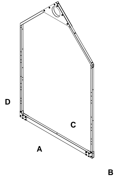
Frame 2 finished part measurements
