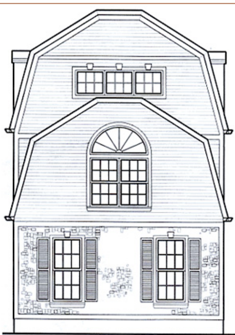
Rear elevation
